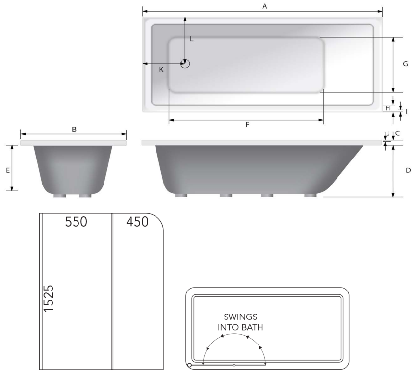
Swing panel swings into bath, providing wide and easy access to bath and tapware.
